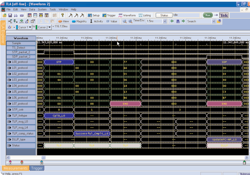
► Figure 32b. Waveform Display of X8 PCI Express Link.
