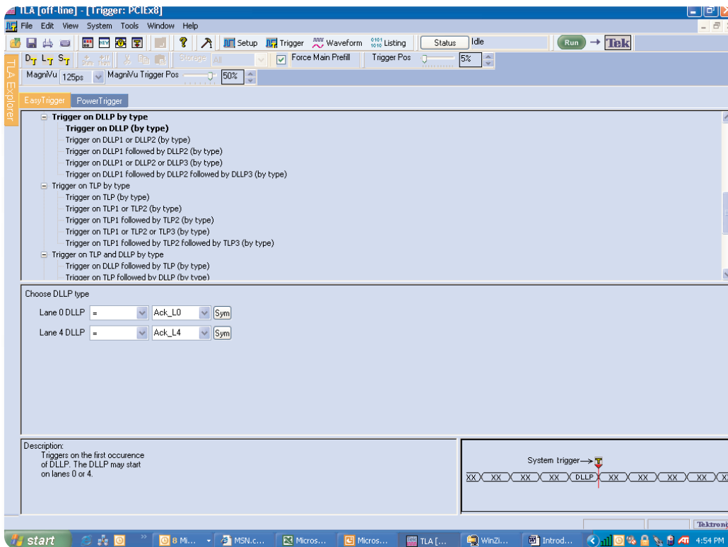
▶ Figure 31. A logic analyzer trigger template.
