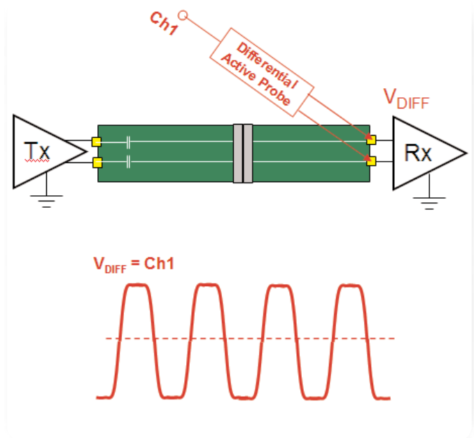
► Figure 21. True Differential Active Probing.
