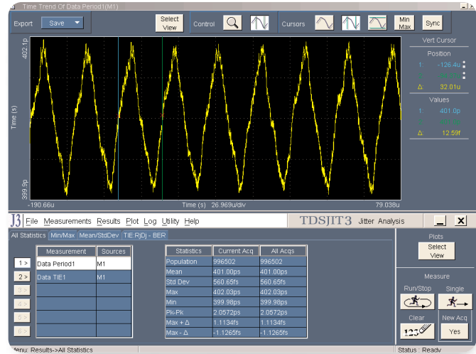
▶ Figure 14. Spread Spectrum Profiling using TDSJIT3 software.
