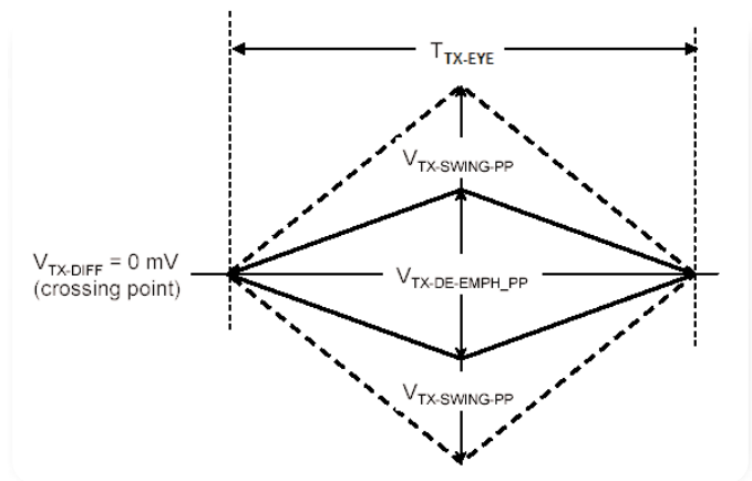
► Figure 15. PCI Express Waveform Mask Specifications.
