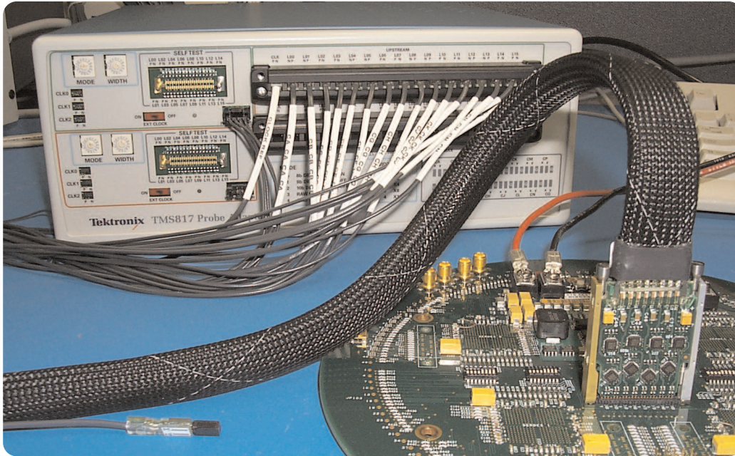
▶ Figure 29. PCI Express Mid-bus probe landing pad.
