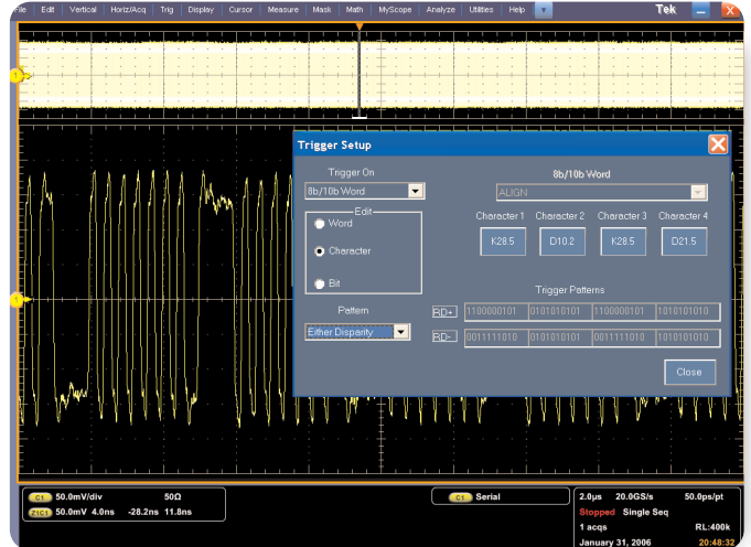
► Figure 27b. Trigger on any combination of four symbols.
