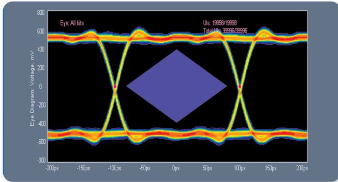
► Figure 25. 5 Gb/s captured with 15GHz oscilloscope.
