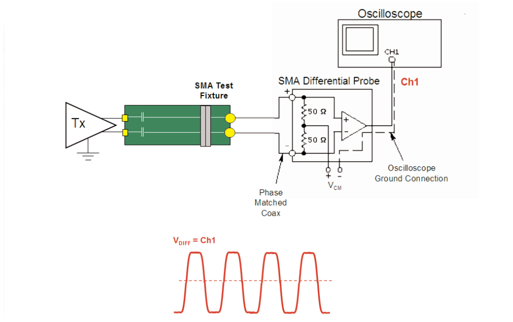
▶ Figure 23. True Differential SMA Probing.
