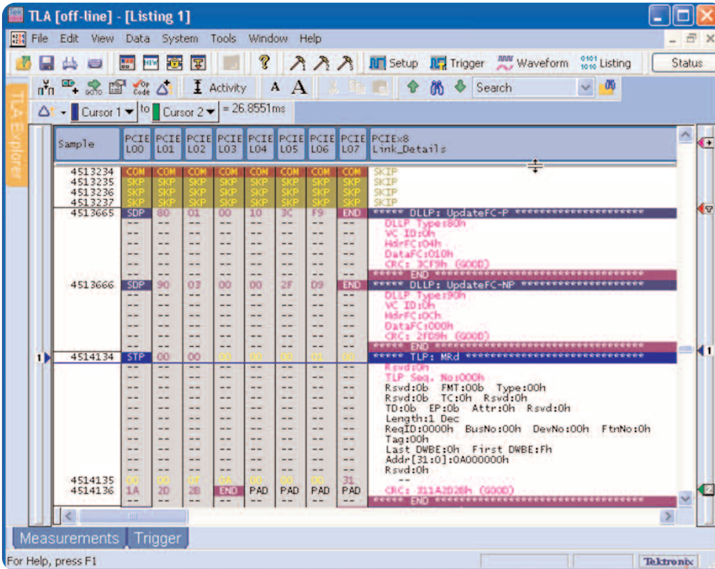
► Figure 32a. Listing Display of X8 PCI Express Link.
