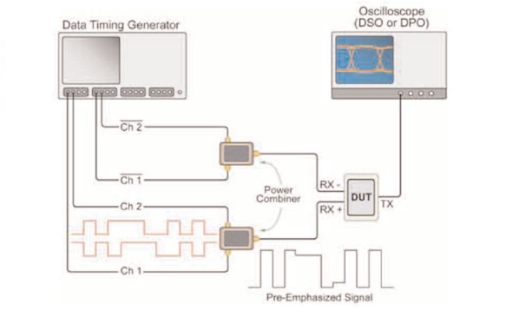
► Figure 18. Creating a de-emphasized signal from two DTG channels.
