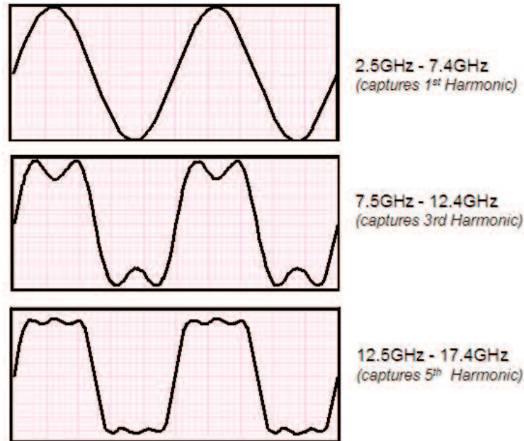
► Figure 24. Pulse response of an ideal low pass filter.
