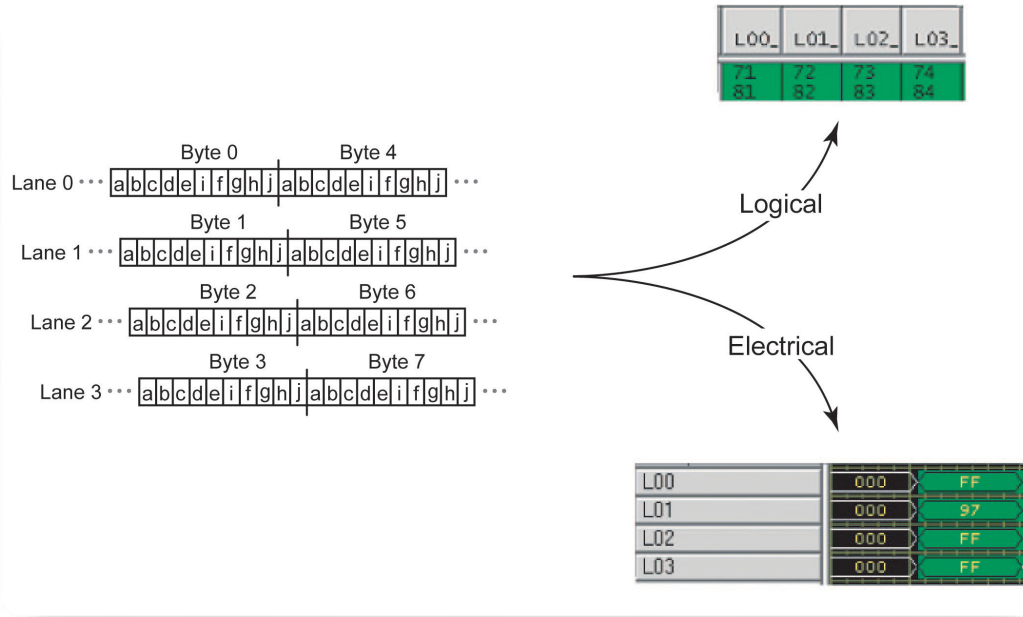
► Figure 30. In this example, the logical view descrambles, deskews, and decodes the data, and sets the bits to the correct polarity. The results are displayed as a stream of hexadecimal data.
