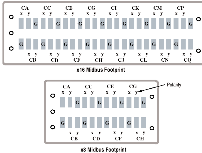
► Figure 28. PCI Express Mid-bus probe landing pad.
