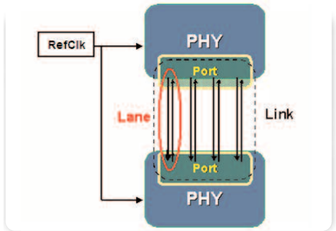
▶ Figure 2. PCI Express PHY link implementation.
